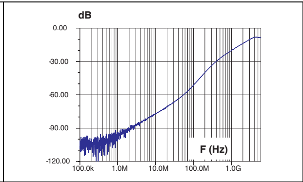
Figure 9. Analog crosstalk measurements between channels
