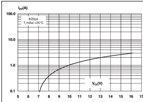
Figure 4. Clamping voltage versus peak pulse current (typical values, 8/20 \mu\text{s} waveform)
