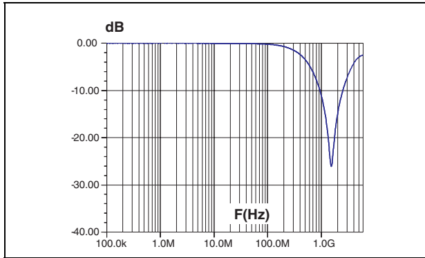
Figure 8. S21 attenuation measurement results of each channel
