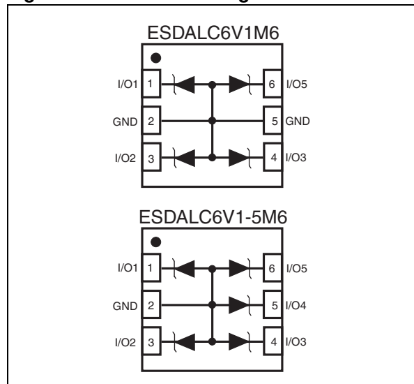
Figure 1. Functional diagram
