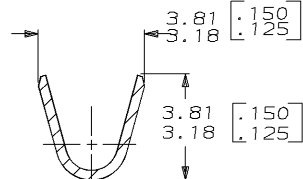
SECTION B-B SCALE 8:1
