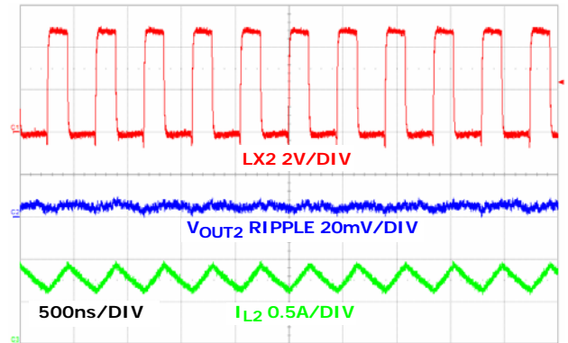
FIGURE 19. STEADY STATE OPERATION WITH FULL LOAD CHANNEL 2
