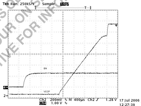
Figure 15. VR11 Startup
