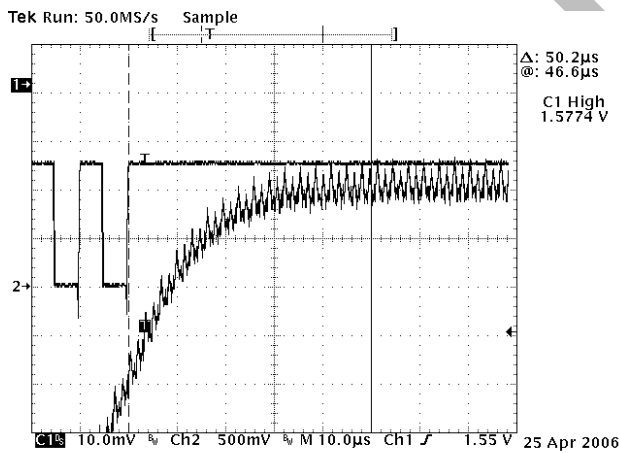
Figure 13. Dynamic VID Settling Time Rising
