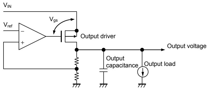
Figure 13 Circuit Diagram
